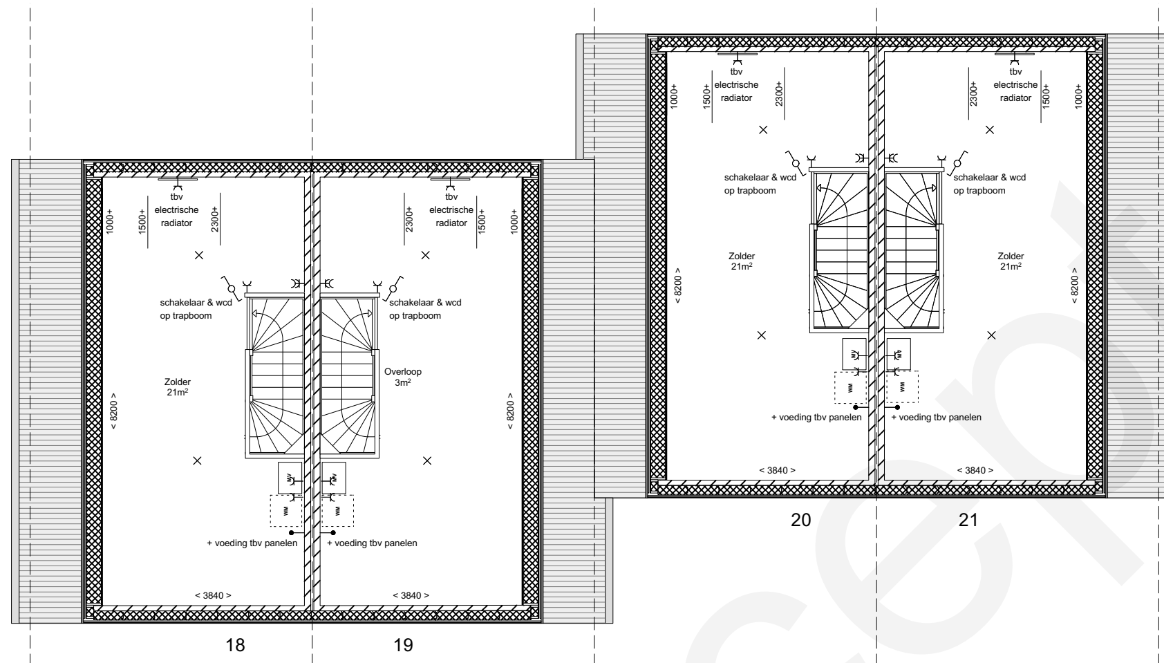
ZOLDER
