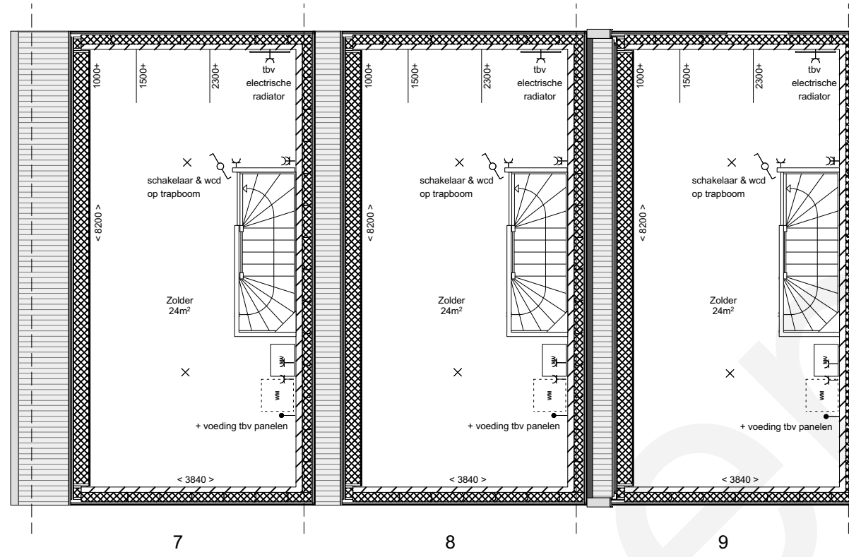
ZOLDER
