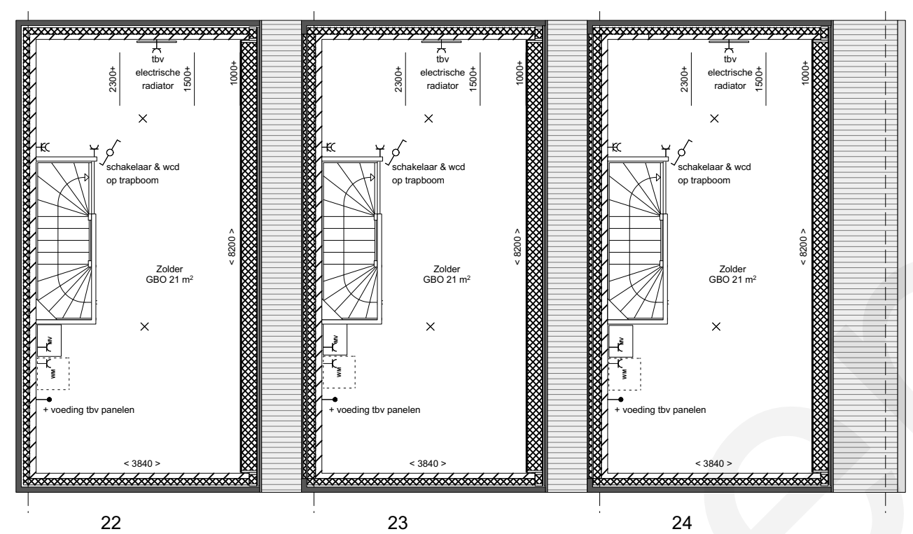
ZOLDER
